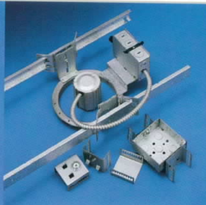
EZ Bar Hanger system for downlights, speaker and fire alarm boxes, exit signs and more, in suspended ceilings.
