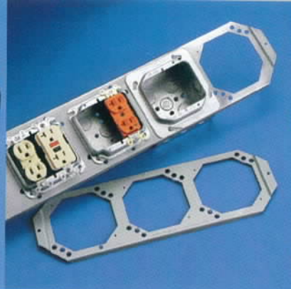
3 & 4 box multiple outlet support brackets for 16" and 24" stud spacing; can be pre-assembled for even easier mounting.
