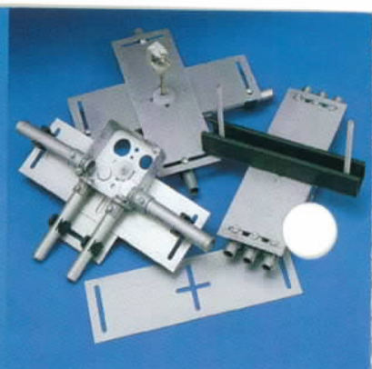
Universal Conduit Support Plate. Support all conduits with same threaded rod or beam clamp used to support the box.
